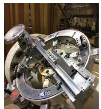
Flange Facing
