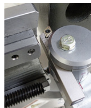
FFR tooling can be adjusted on multiple axes
