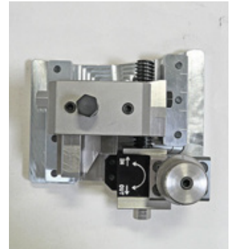
Slides accept 1in (25.4mm) square & all popular size tooling
