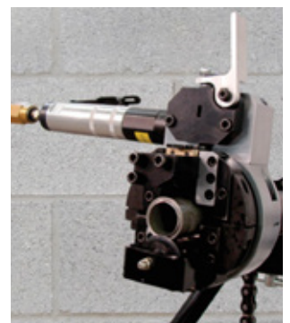
FME Wheel Cutting
