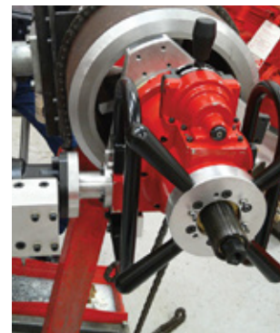
EP 424 AutoFeed deluxe beveling with form tool rotating head
