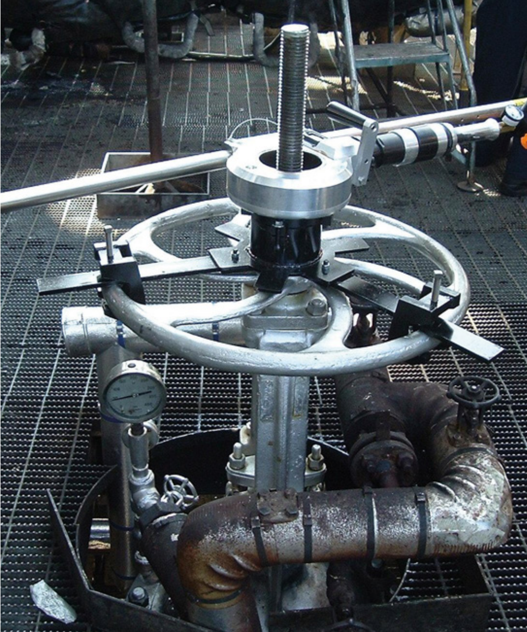
Handheld powered valve operators
