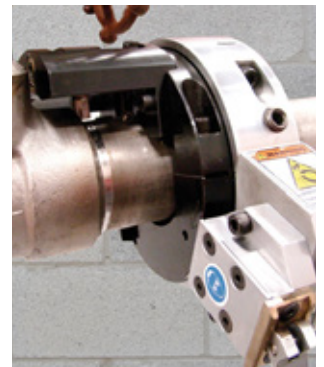
Socket Weld Removal
