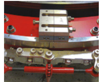
Swing bolts & hinge mechanism speeds assembly & mounting
