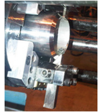
SDSF Cut & Bevel
