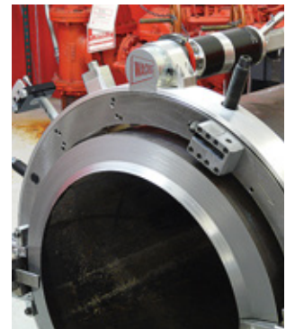
Base Kits come complete, just add drive motor and tooling
